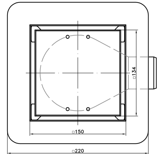
150 x 150 mm Designrost Pure Siphon H+M Drop 50
