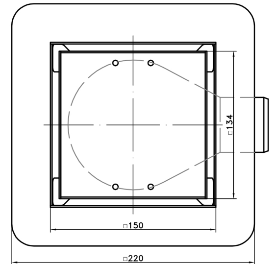
150 x 150 mm Designrost Pure Siphon H+M Drop 35
